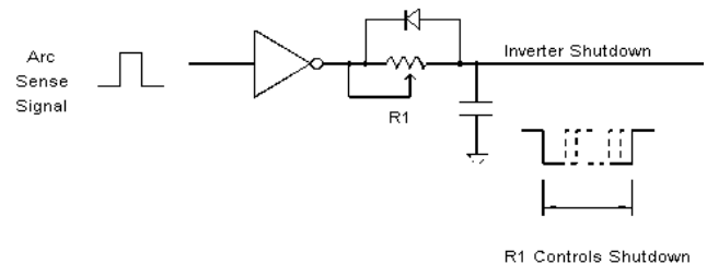
Fig. 4 Arc Quench
