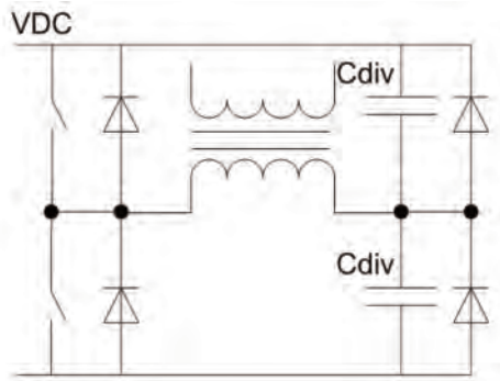
Fig. 2. Inverter with energy dosing capacitors
