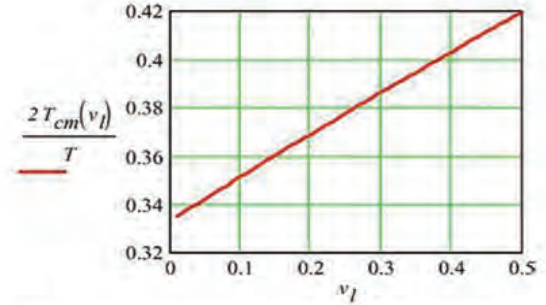
Fig. 26. Worst chopping moment versus normalized load voltage.
