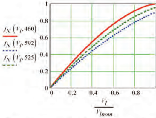
Fig. 3. ZCC curves for low (460 V), high (592 V), and nominal (525 V) dc rail voltages. V_{Lnom} is nominal load voltage.
