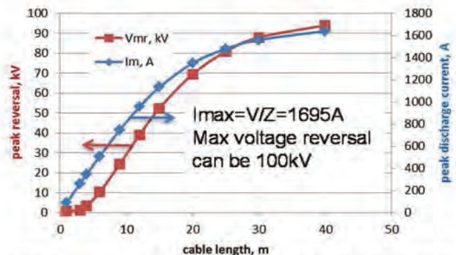
Figure 2. Dependence of peak reversal voltage and peak discharge current (V(T1:A+) and IB(T1), respectively, per notation of Figure 1) on cable length (referenced to charge voltage of 100 kV). In these simulations, TTRAN=1 \mu s (actual transition from 90% to 10% is 200ns).
