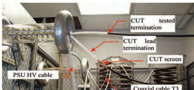
Figure 2. Experimental setup.
